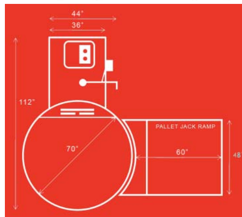
Plan View
