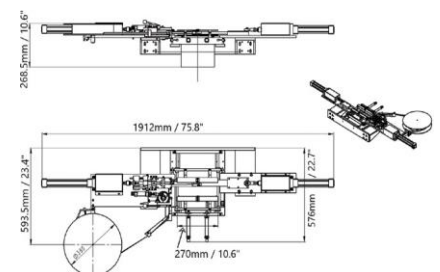
CLIPPING MACHINE LAYOUT
